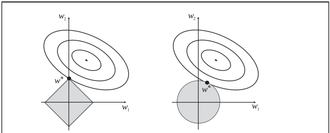
Figure 18.14 Why L_1 regularization tends to produce a sparse model. (a) With L_1 regu-
