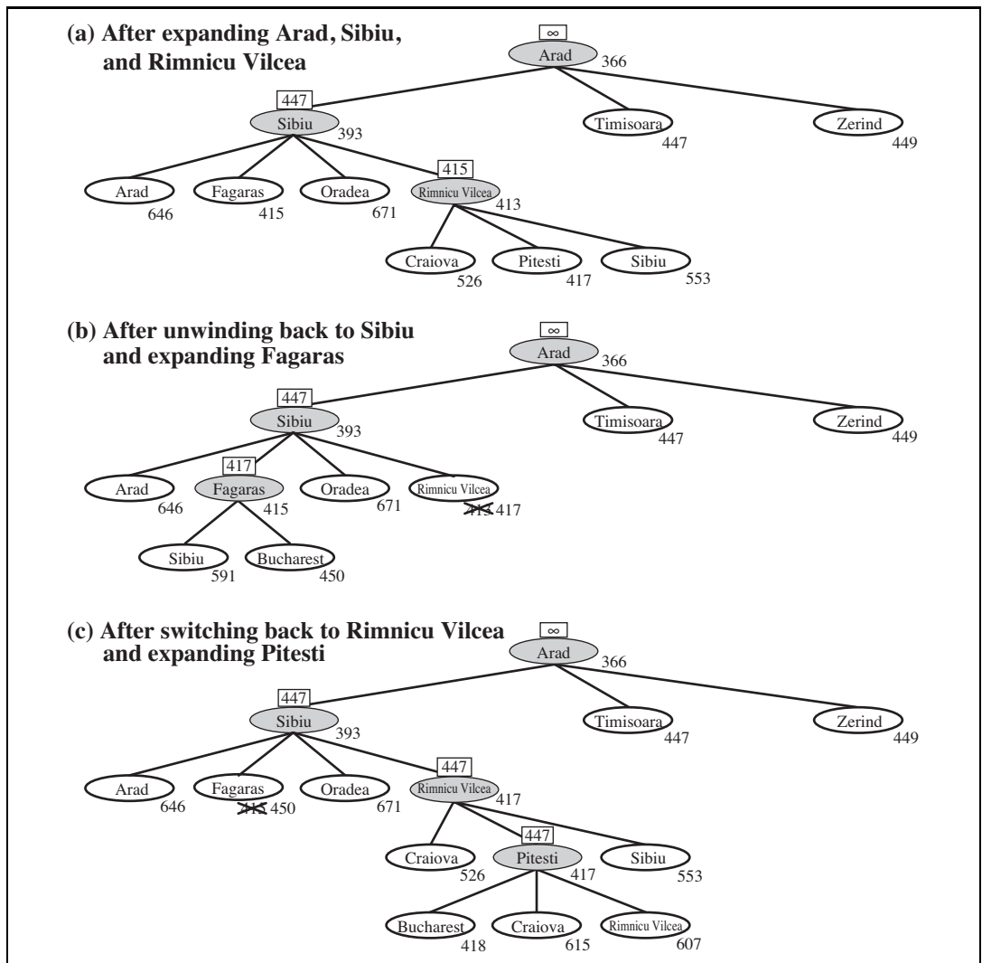
Figure 3.27 Stages in an RBFS search for the shortest route to Bucharest. The f-limit value for each recursive call is shown on top of each current node, and every node is labeled with its f-cost. (a) The path via Rimnicu Vilcea is followed until the current best leaf (Pitesti) has a value that is worse than the best alternative path (Fagaras). (b) The recursion unwinds and the best leaf value of the forgotten subtree (417) is backed up to Rimnicu Vilcea; then Fagaras is expanded, revealing a best leaf value of 450. (c) The recursion unwinds and the best leaf value of the forgotten subtree (450) is backed up to Fagaras; then Rimnicu Vilcea is expanded. This time, because the best alternative path (through Timisoara) costs at least 447, the expansion continues to Bucharest.
